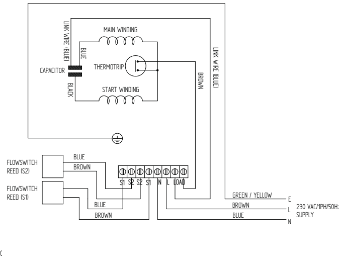
Twin Pumps Fig. 14
