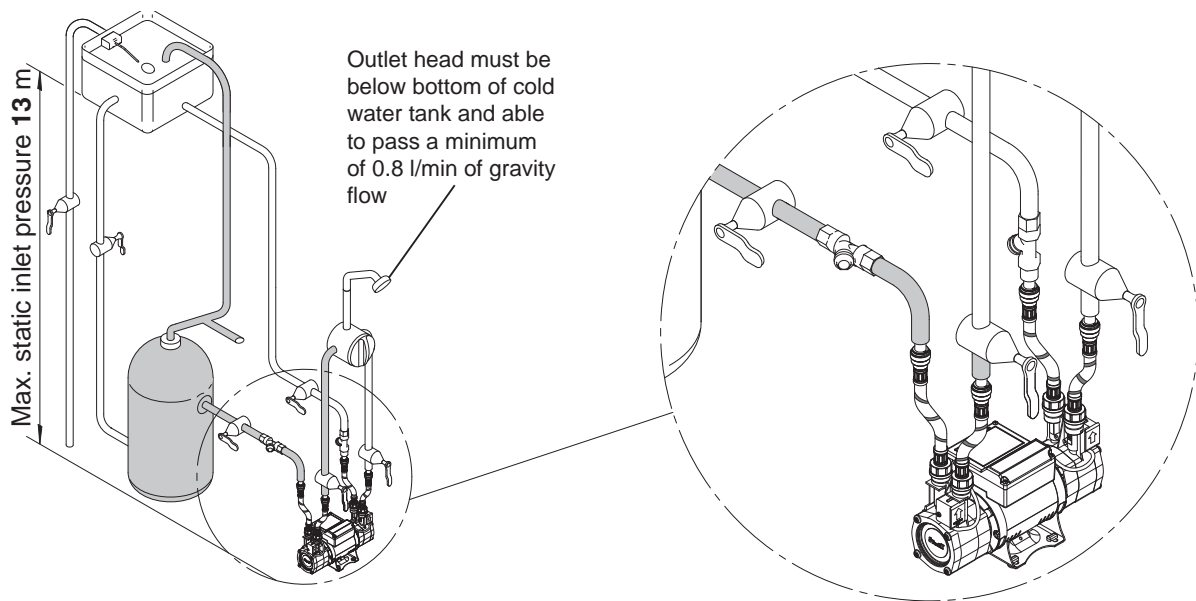
Twin Pump System Fig. 5
