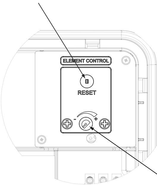
THERMAL CUT-OUT RESET BUTTON
