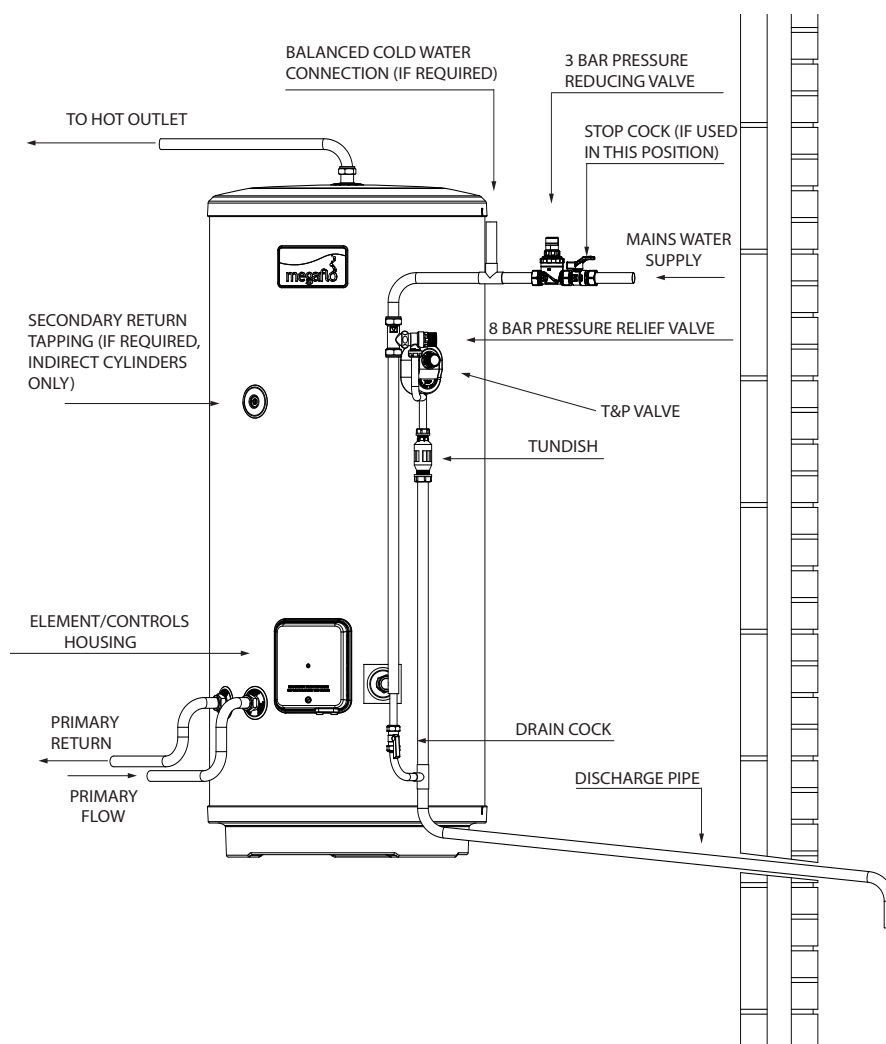
Figure 1 - Schematic Installation Details
