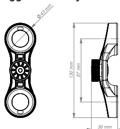
Trigger assembly
