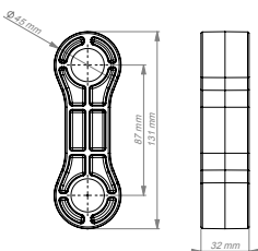
Alignment jig
