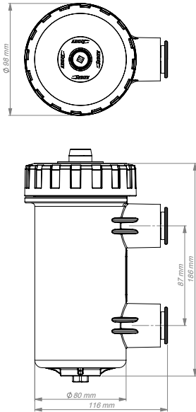
Canister
