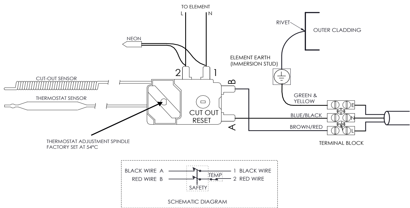
Figure 2: Wiring Diagram
